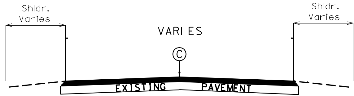
TYPICAL SECTION NO. 1
