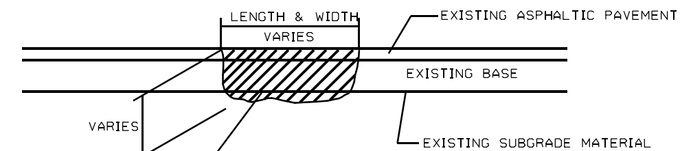
DETAIL D PATCHING EXISTING PAVEMENT
