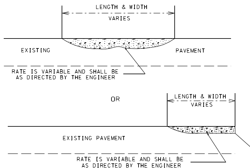
DETAIL B ASPHALT CONCRETE SURFACE COURSE TYPE S9.5B. (LEVELING COURSE)
